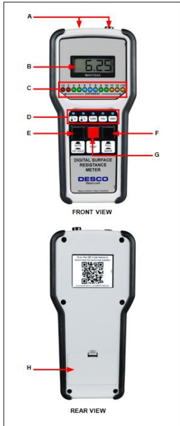
Figure 4. Digital Surface Resistance Meter features and components
